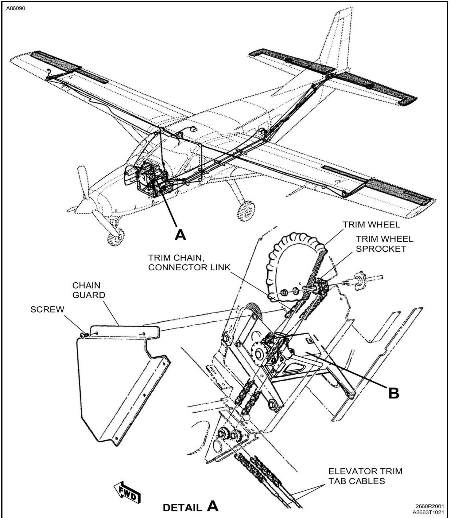
Figure 401 : Sheet 1 : Autopilot Pitch Trim Servo Installation
